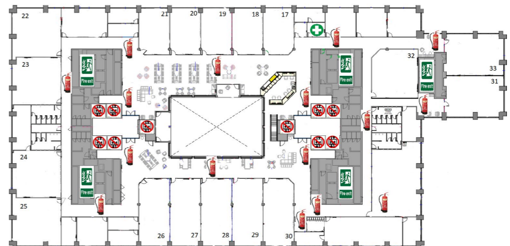
Import building 4th floor
